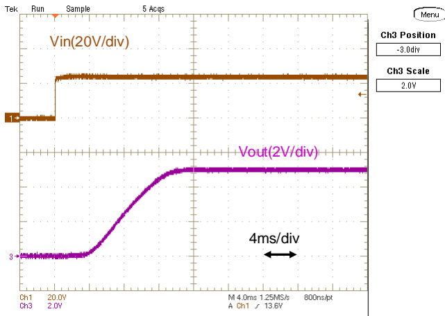
Fig.12-2-7. Start-up Waveform (Io=0A)
