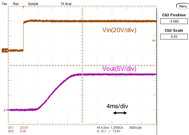
Fig.12-2-31. Start-up Waveform (Io=0A)
