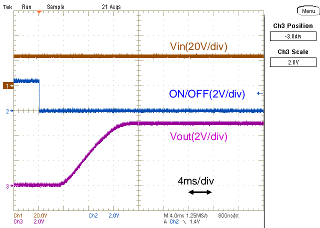
Fig.12-2-9. Start-up Waveform (Io=0A)
