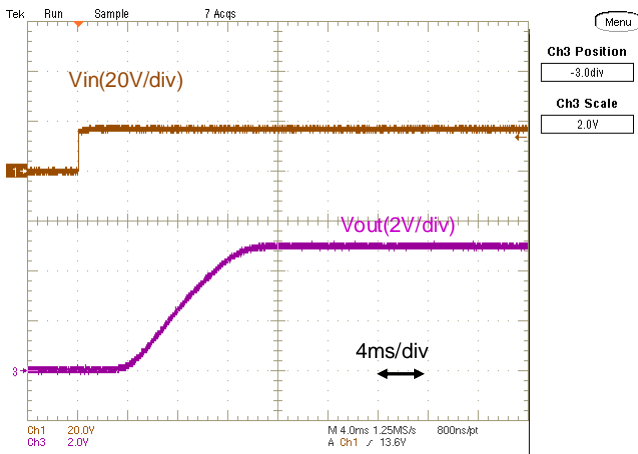
Fig.12-2-1. Start-up Waveform (Io=0A)
