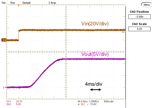
Fig.12-2-19. Start-up Waveform (Io=0A)
