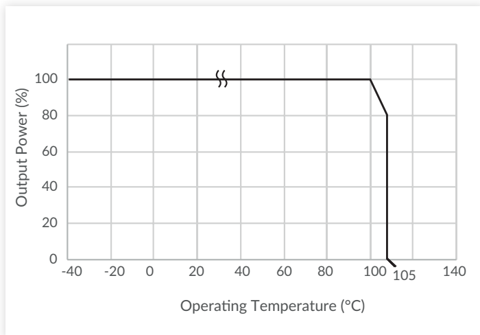
Thermal Derating Curve
