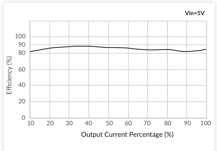
Efficiency vs Output Load (IAS0105D05)
