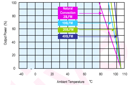
MJWI15-48S033 Derating Curve with Heatsink
