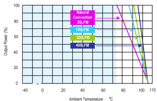
MJWI15-24S05, MJWI15-24S12, MJWI15-48S05 Derating Curve with Heatsink
