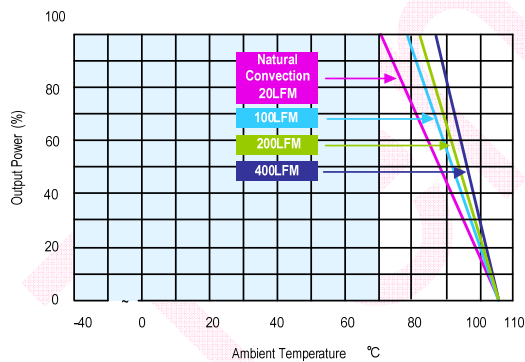
MJWI15-24S15, MJWI15-24D12, MJWI15-24D15, MJWI15-48S12, MJWI15-48S15, MJWI15-48D15 Derating Curve without Heatsink
