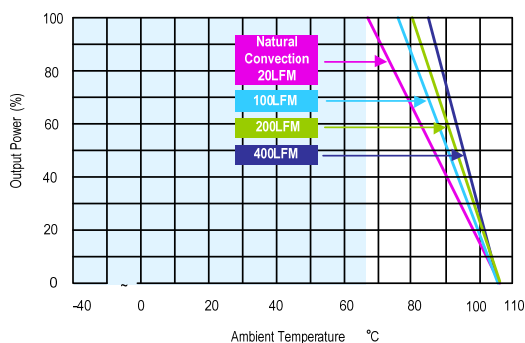
MJWI15-24S05, MJWI15-24S12, MJWI15-48S05 Derating Curve without Heatsink
