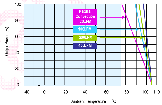
MJWI15-24S033 Derating Curve with Heatsink
