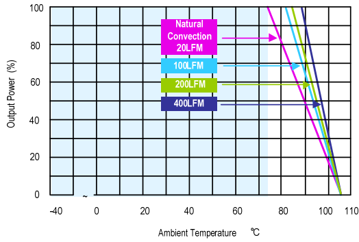
MJWI15-48S033 Derating Curve without Heatsink
