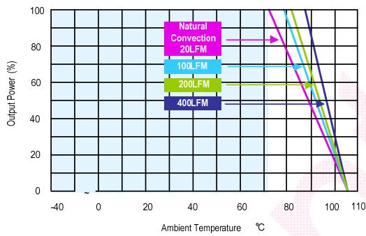
MJWI15-24S033 Derating Curve without Heatsink
