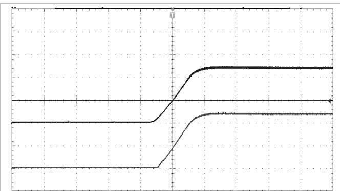
Start-up, enabled by connecting V_i at: T_{P1} = +25^\circ\text{C} , V_i = 12\text{ V} , V_o = 5\text{ V} I_o = 200\text{ mA} resistive load.
