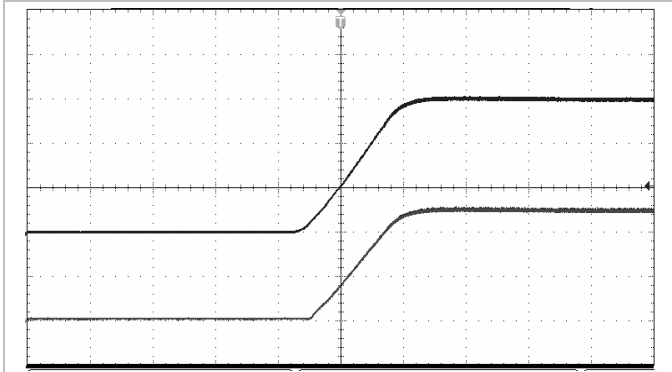
Start-up, enabled by connecting V_i at: T_{P1} = +25^\circ\text{C} , V_i = 15\text{ V} , V_o = 5\text{ V} I_o = 200\text{ mA} resistive load.
