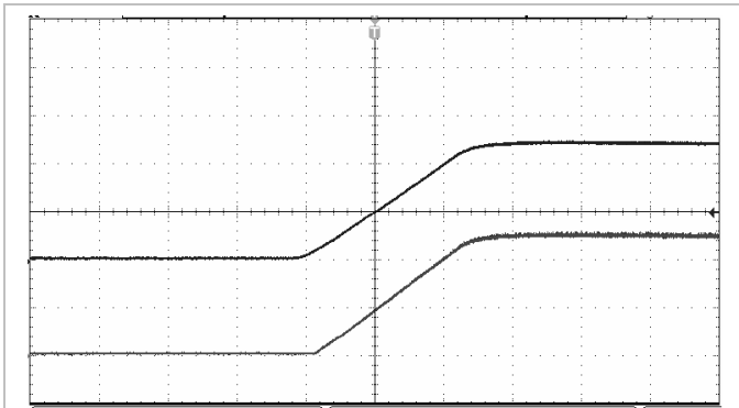
Start-up, enabled by connecting V_i at: T_{P1} = +25^\circ\text{C} , V_i = 24\text{ V} , V_o = 5\text{ V} I_o = 200\text{ mA} resistive load.
