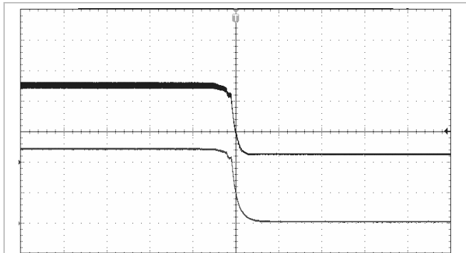
Start-up, enabled by connecting V_i at: T_{P1} = +25^\circ\text{C} , V_i = 5\text{ V} , V_o = 5\text{ V} I_o = 200\text{ mA} resistive load.
