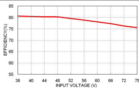
PDS02-48S05 Efficiency vs. Input Voltage
