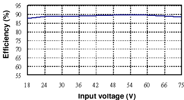
BUC20-48S1W Input voltage vs. Efficiency
