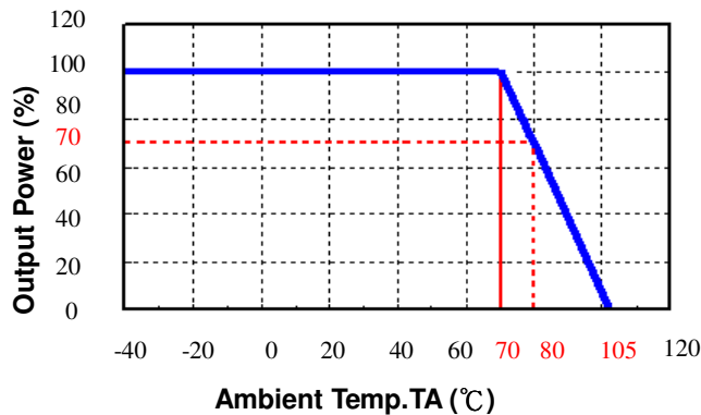
BUC20W Series Power Derating Curve(5)
