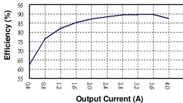
BUC20-48S1W Output Current vs. Efficiency
